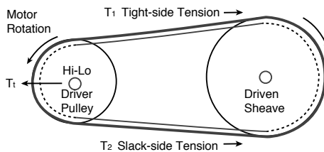
Tension Force Direction
