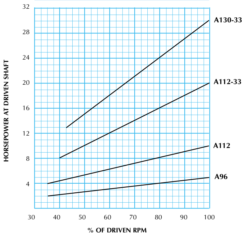
Horsepower Curve (1750 RPM Input)
