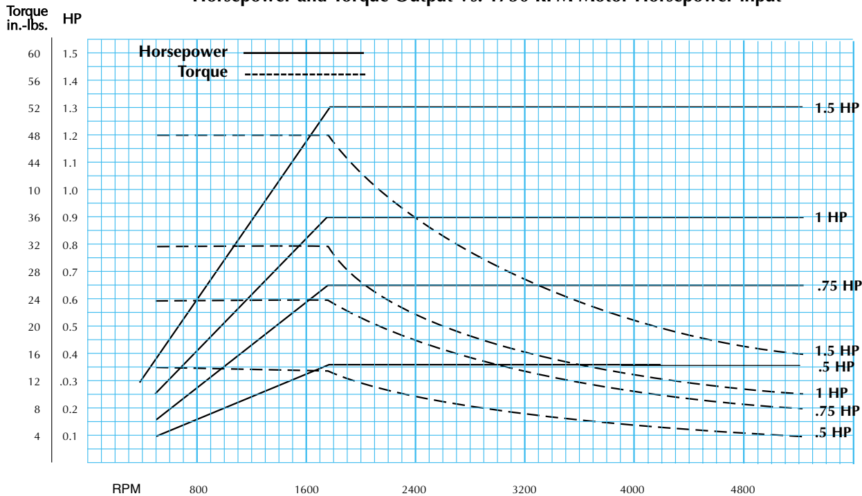
Model 6060 VARI-Mod Horsepower and Torque Output Vs. 1750 RPM Motor Horsepower input
