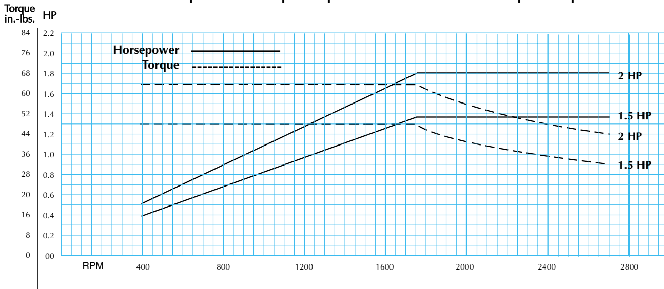
Model 6075 VARI-Mod Horsepower and Torque Output Vs. 1750 RPM Motor Horsepower input
